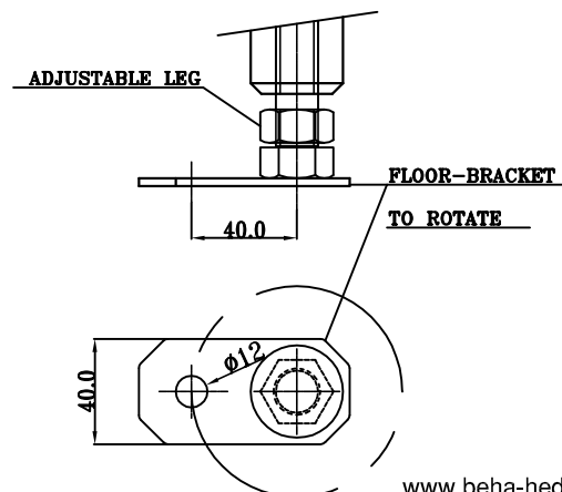
FLOOR FASTENING DETAIL
